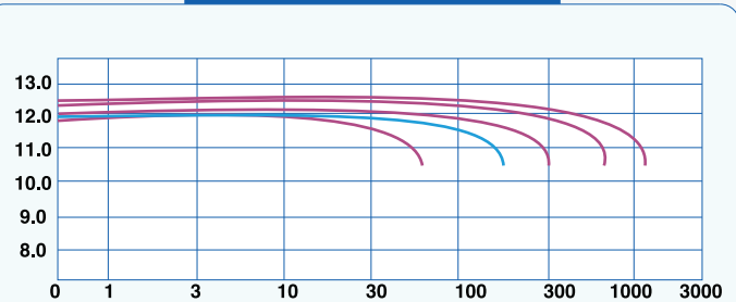
Discharging Characteristics
