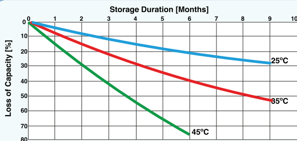
Self Discharge Characteristics - Tubular Batteries
