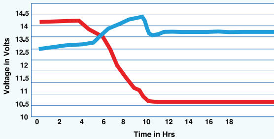
Charging Characteristics
