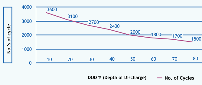
Cycle Life Vs DOD
